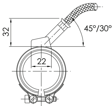
Tangential exit 30°/45°
